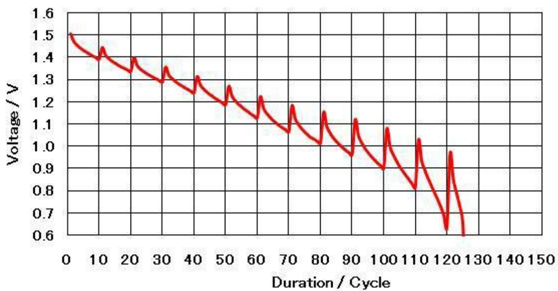
Digital still camera : (1500mW 2sec. on/650mW 28sec. on ) *10/hr
